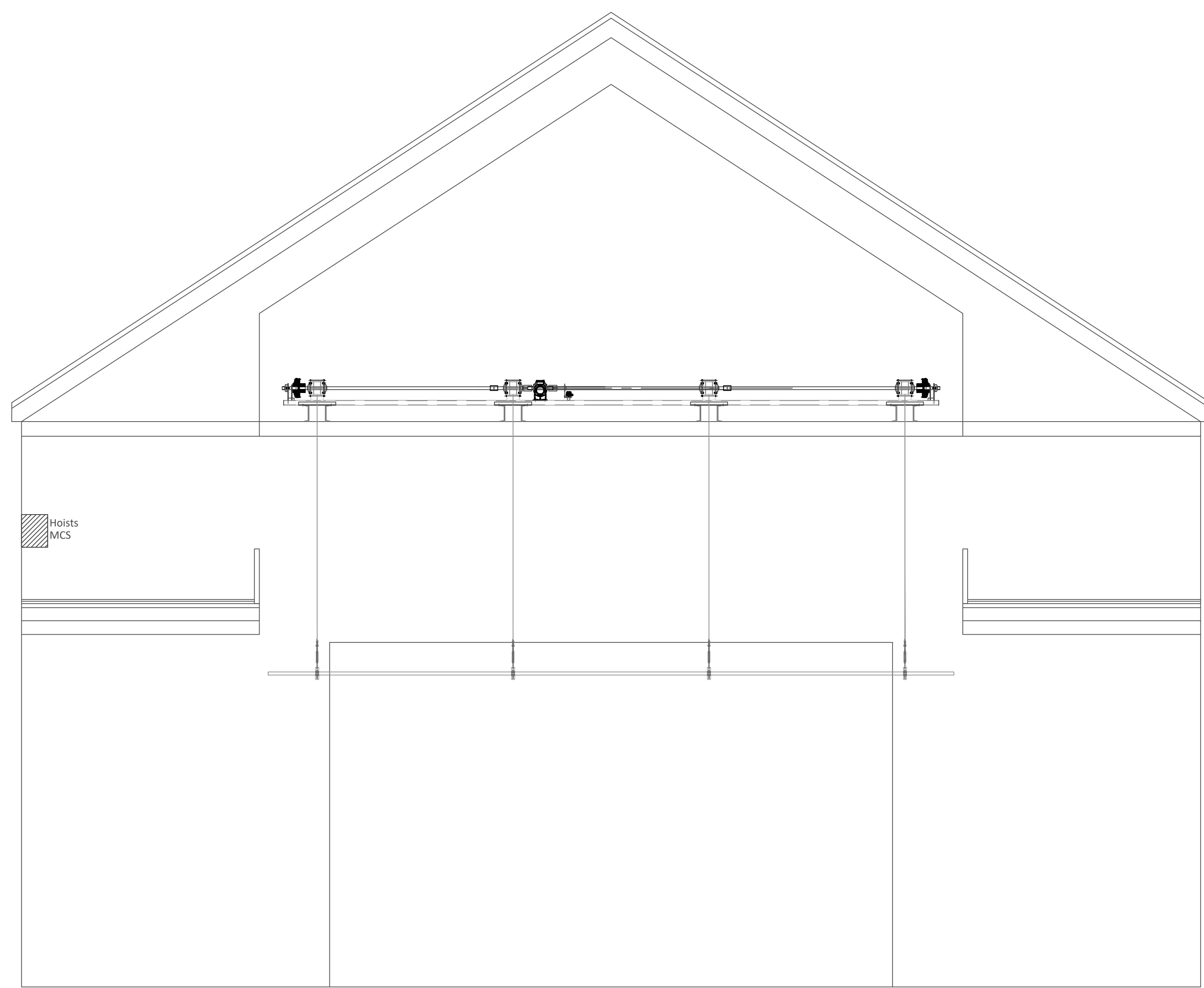
LINE SHAFT HOIST ELEVATION SCALE: 1/4"=1'-0"
