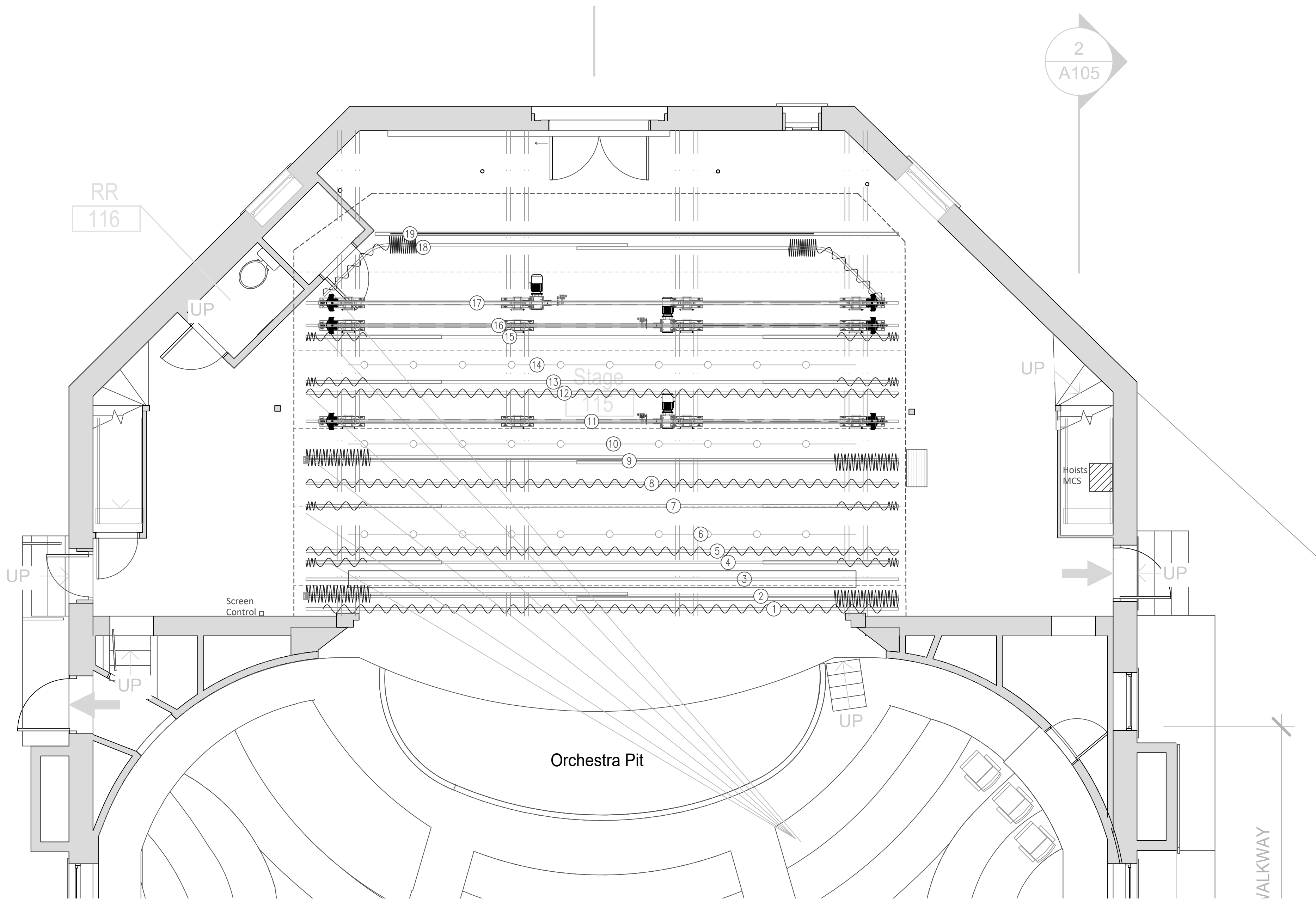
STAGE PLAN SCALE: 1/4"=1'-0"
